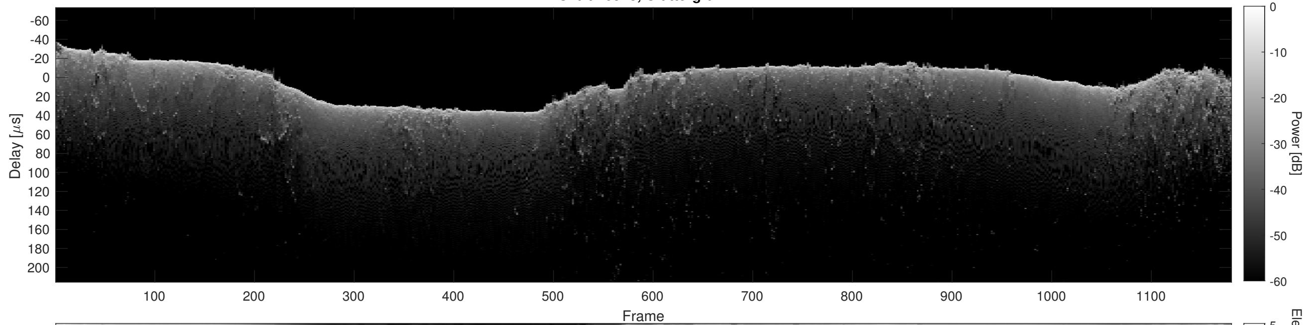
Orbit 20918, Cluttergram
