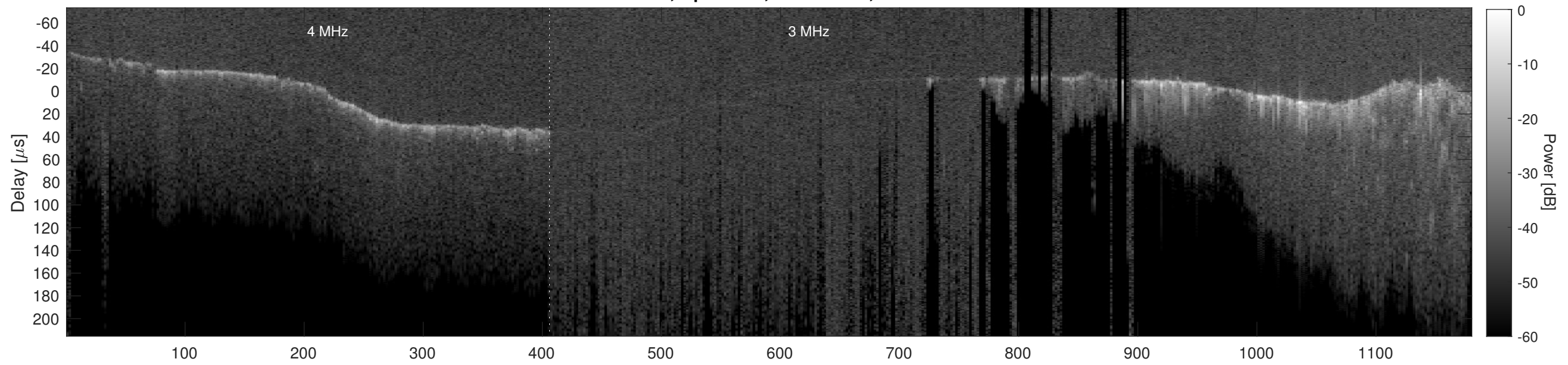
Orbit 20918, Cluttergram
