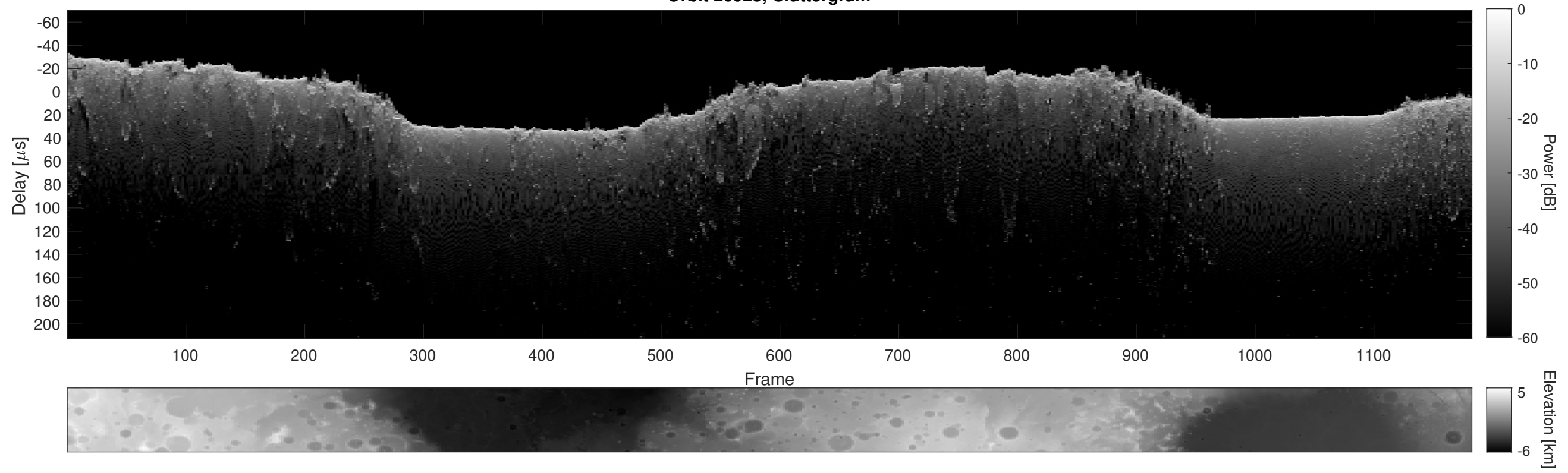
Orbit 20925, Cluttergram
