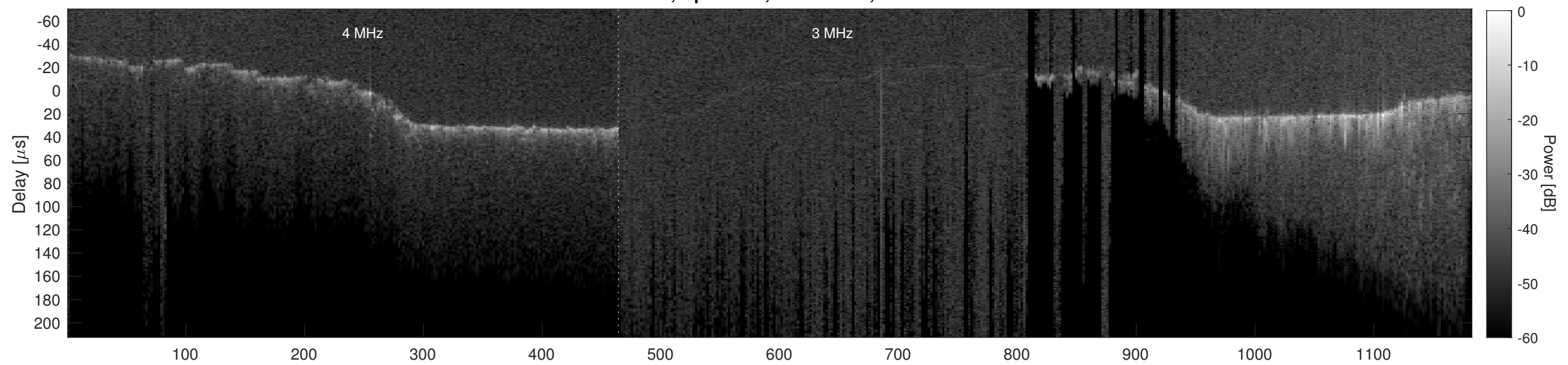
Orbit 20925, Cluttergram
