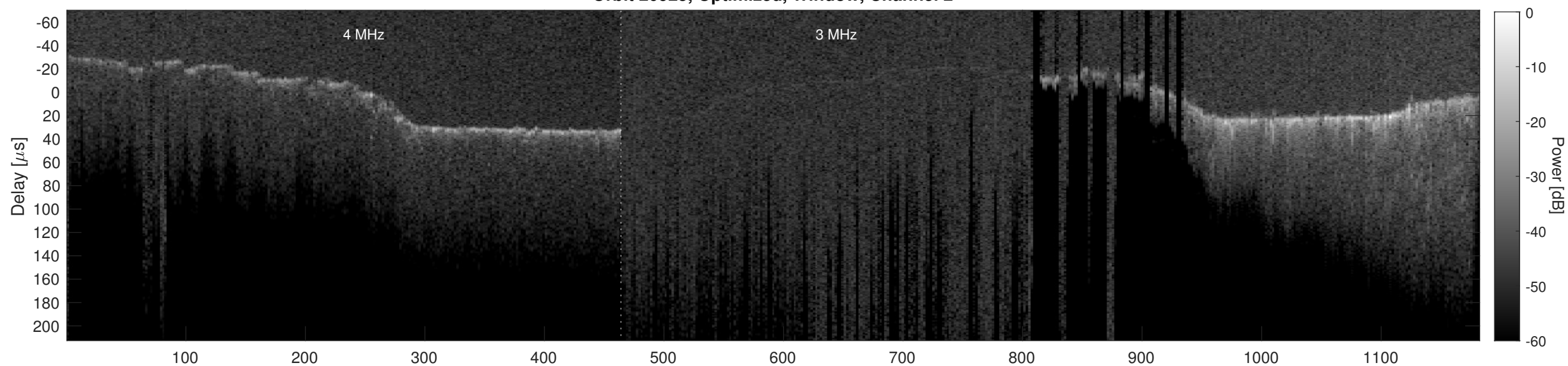
Orbit 20925, Cluttergram
