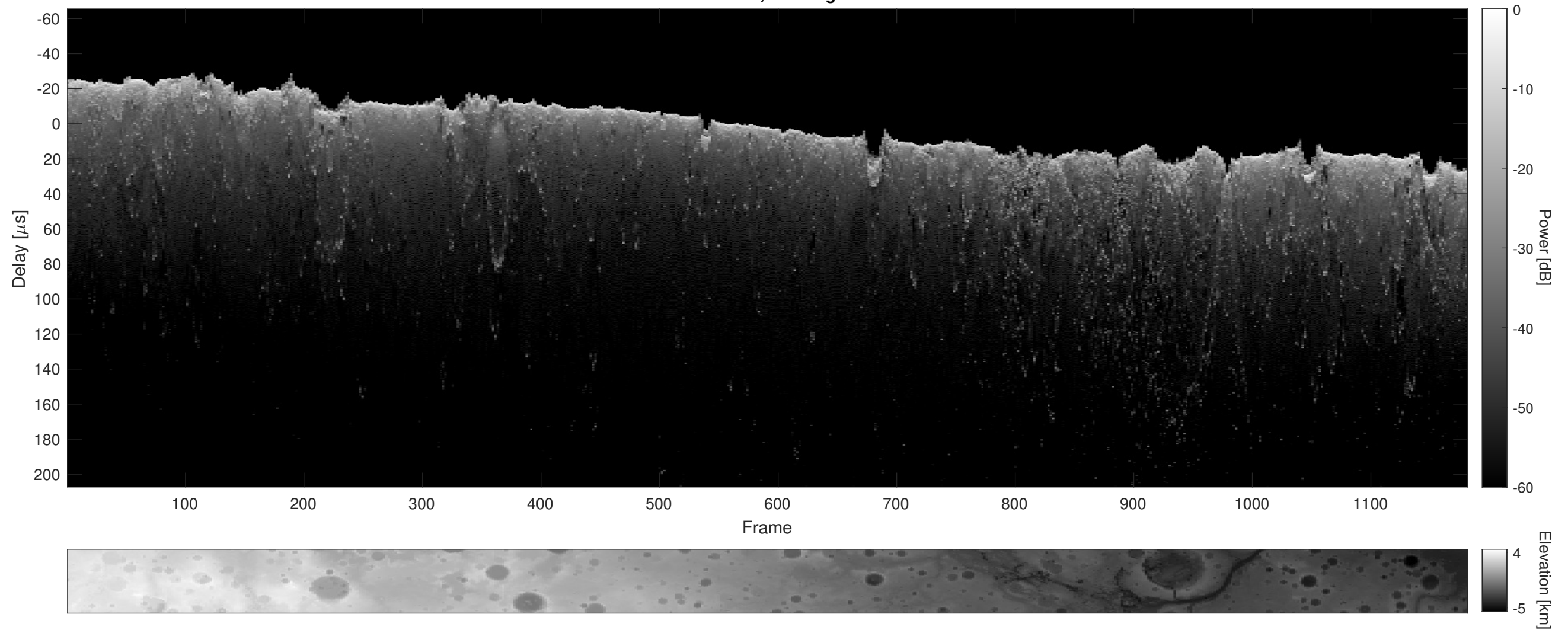
Orbit 20926, Cluttergram
