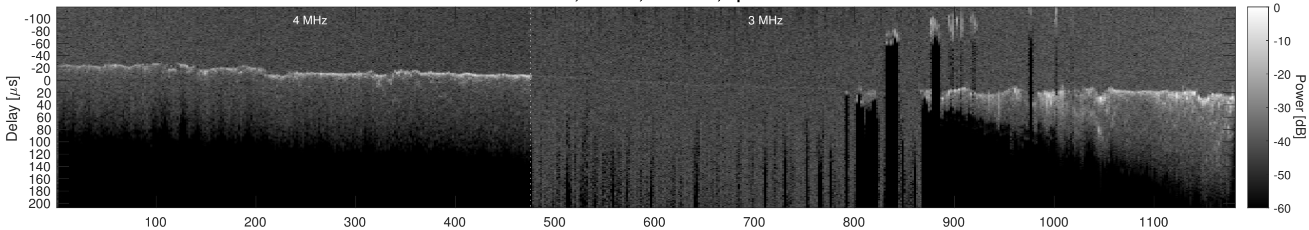
Orbit 20926, Cluttergram
