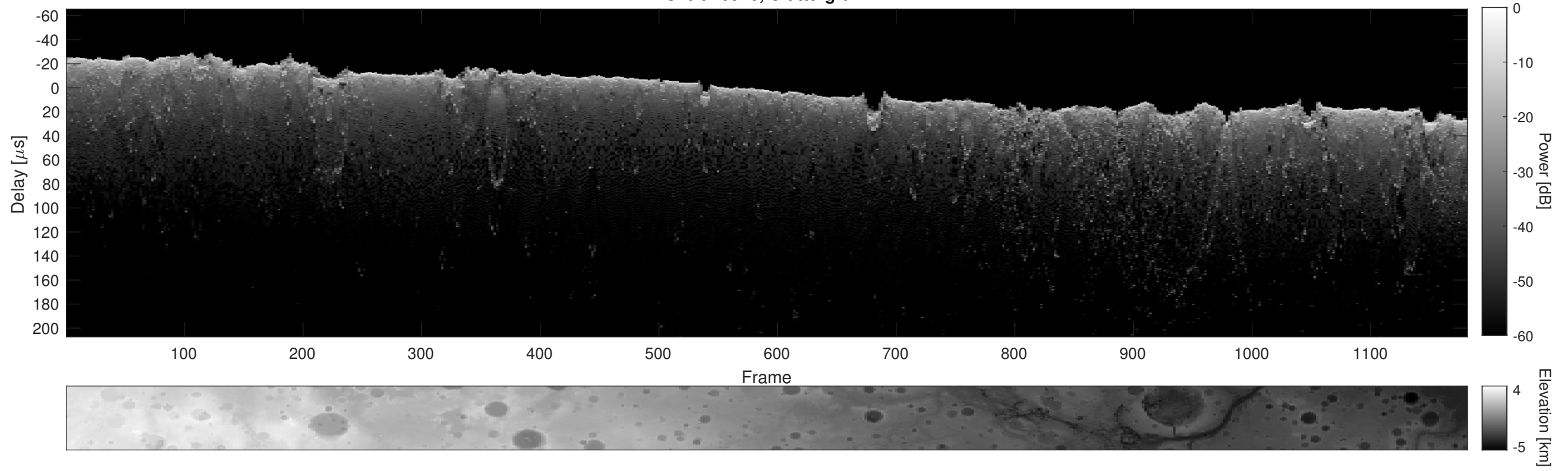
Orbit 20926, Cluttergram
