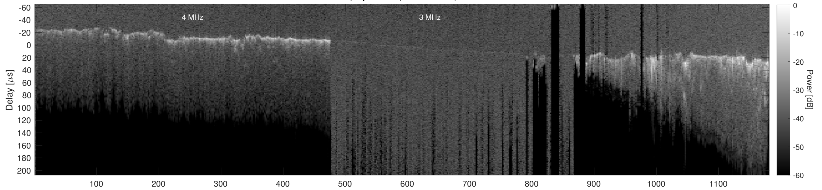
Orbit 20926, Cluttergram
