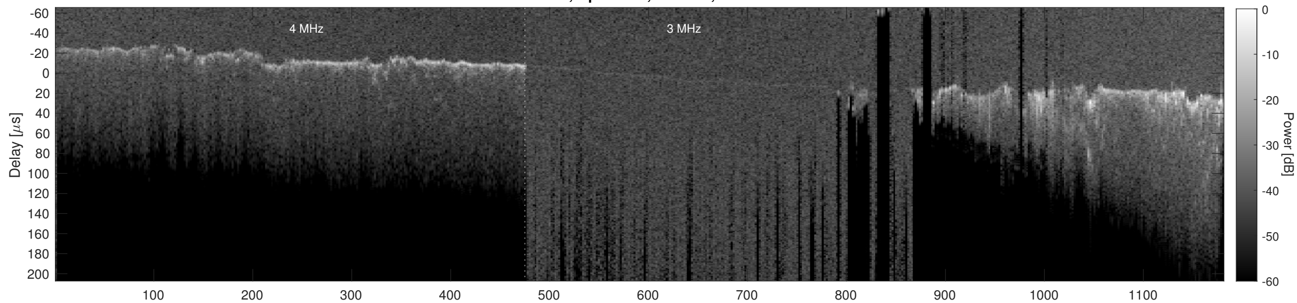
Orbit 20926, Cluttergram
