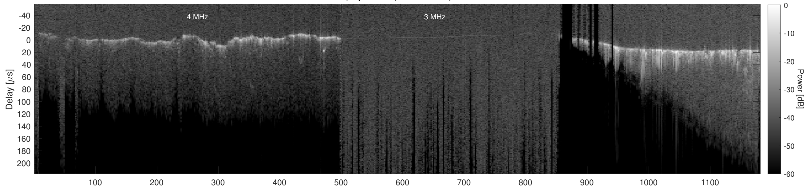
Orbit 20930, Cluttergram
