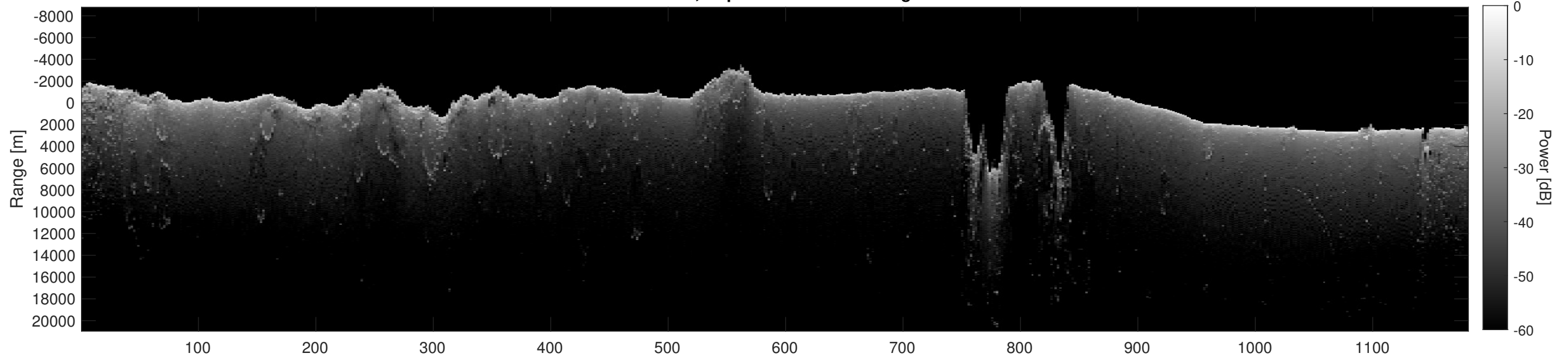
Orbit 20930, Depth-Corrected Cluttergram
