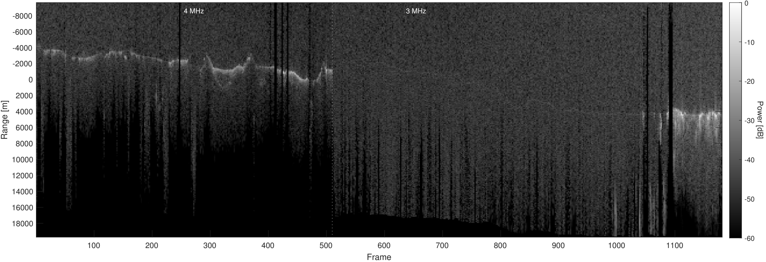
Orbit 20931, Optimized, No Window, Depth-Corrected, Channel 2
