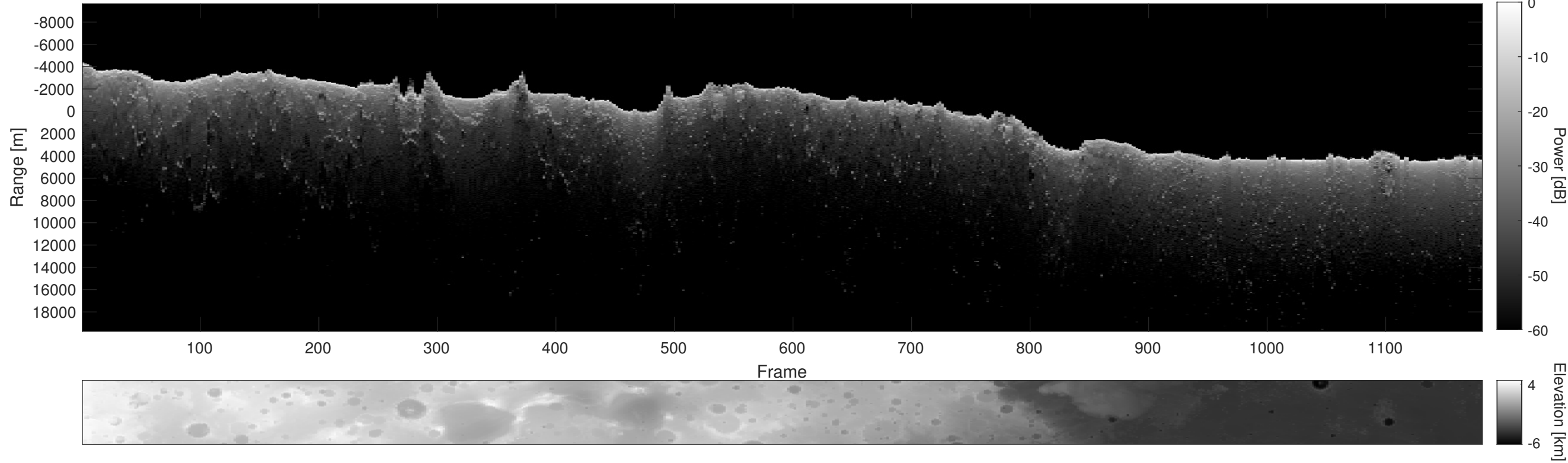
Orbit 20931, Depth-Corrected Cluttergram
