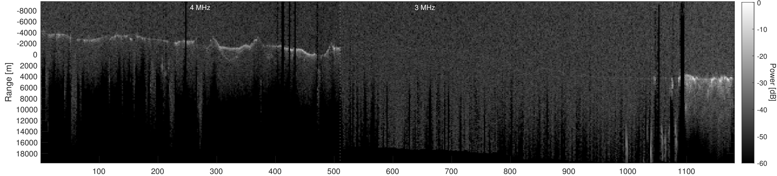
Orbit 20931, Depth-Corrected Cluttergram
