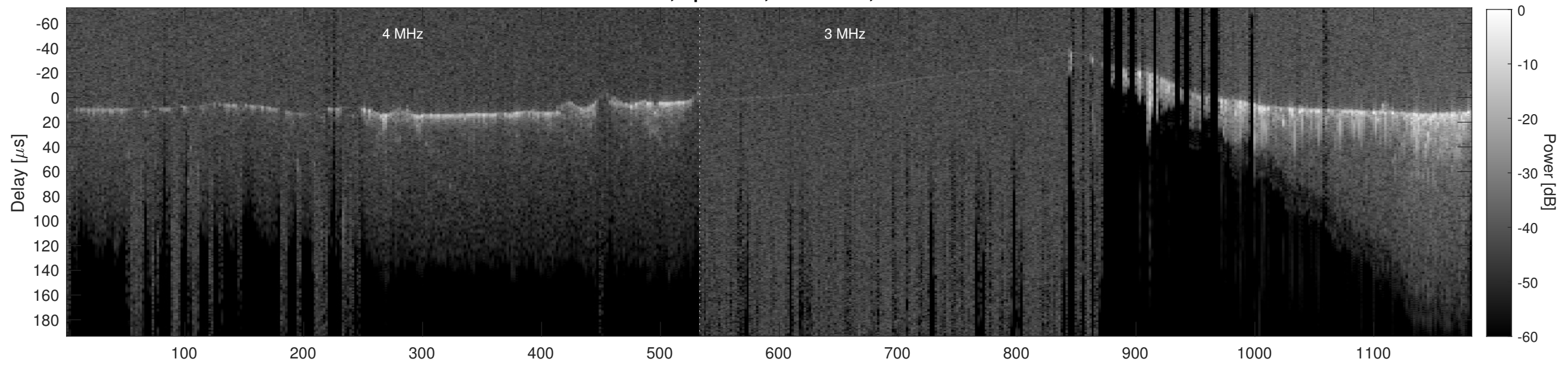
Orbit 20934, Cluttergram
