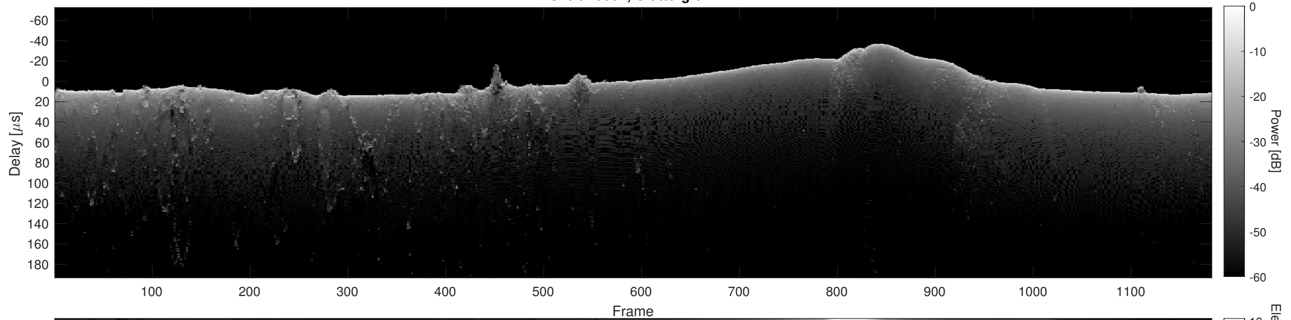
Orbit 20934, Cluttergram
