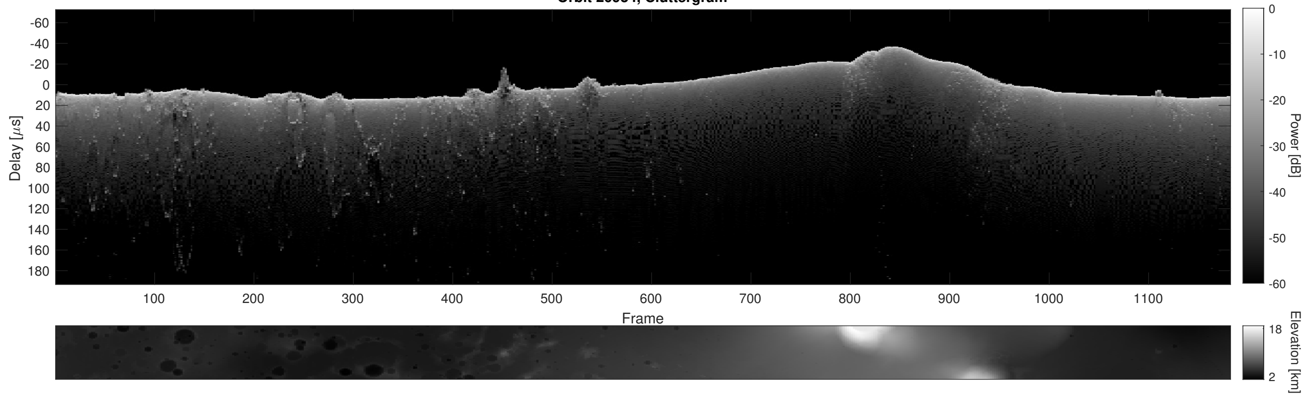
Orbit 20934, Cluttergram
