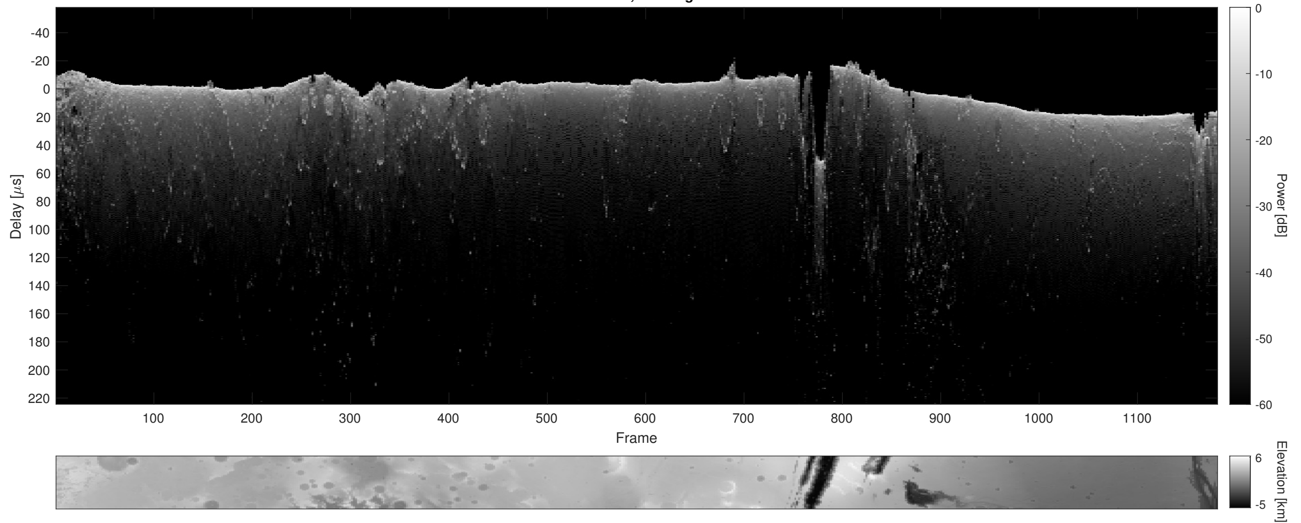
Orbit 20937, Cluttergram
