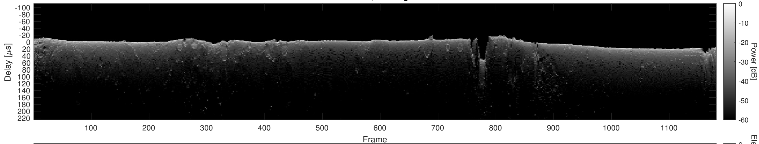
Orbit 20937, Cluttergram
