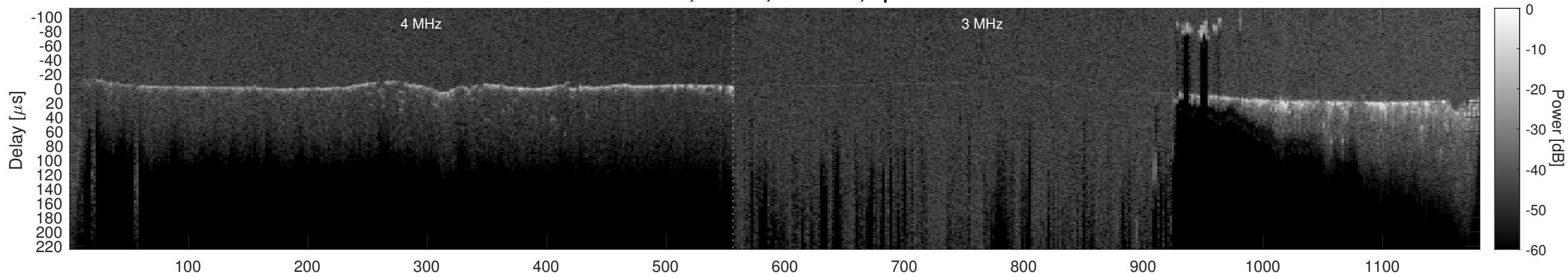
Orbit 20937, Cluttergram
