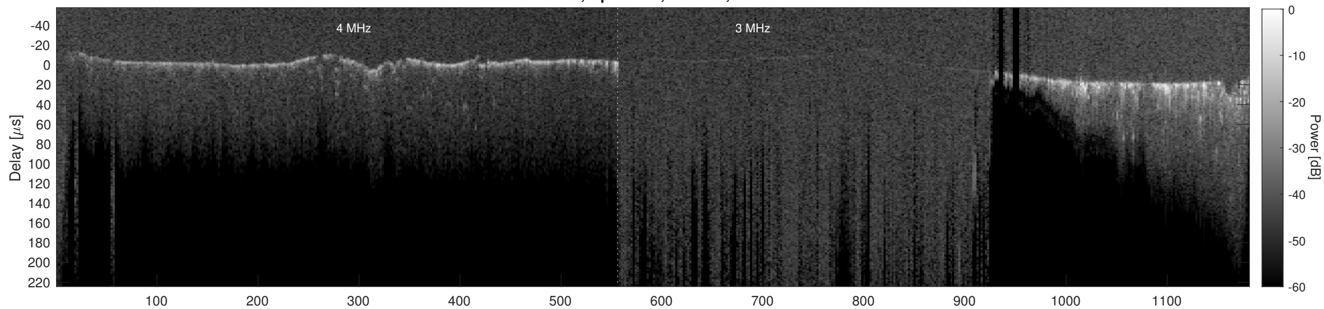
Orbit 20937, Cluttergram
