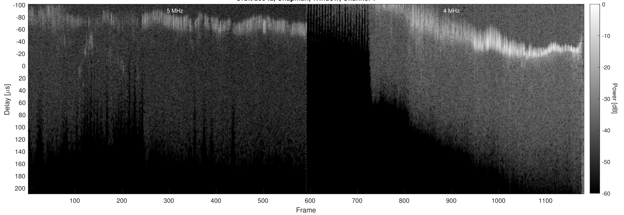
Orbit 20942, Chapman, Window, Channel 2
