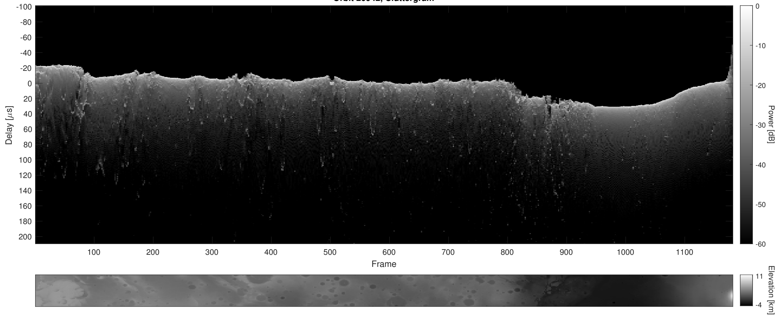
Orbit 20942, Cluttergram
