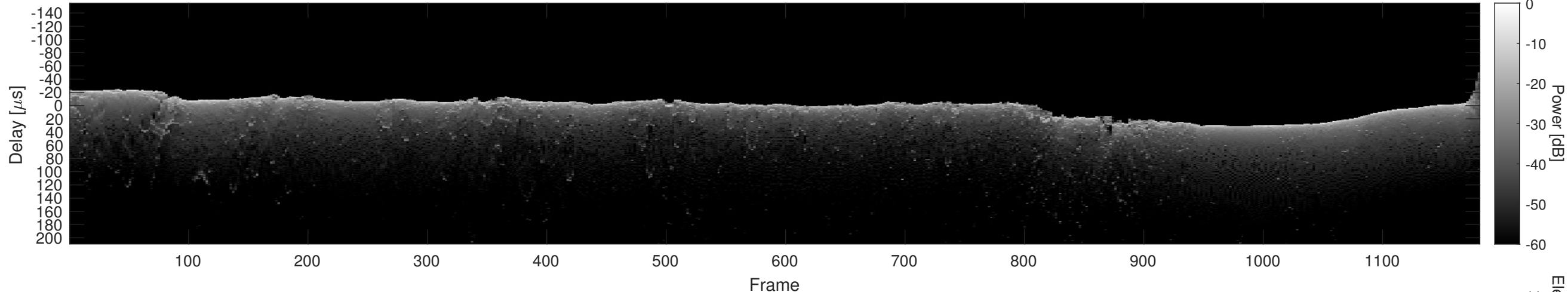
Orbit 20942, Cluttergram
