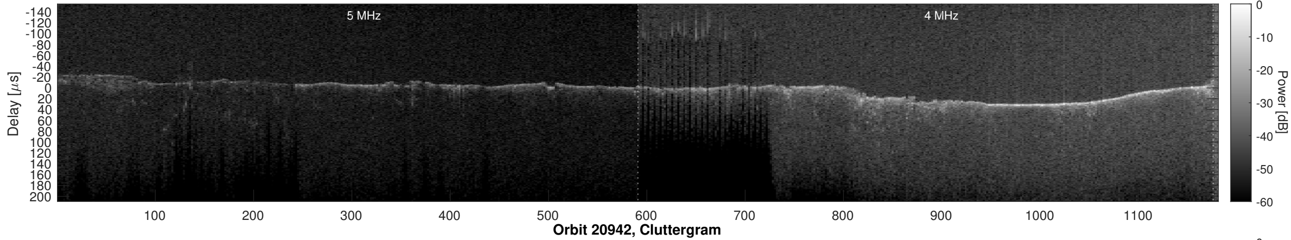
Orbit 20942, Window, Channel 1, Optimized
