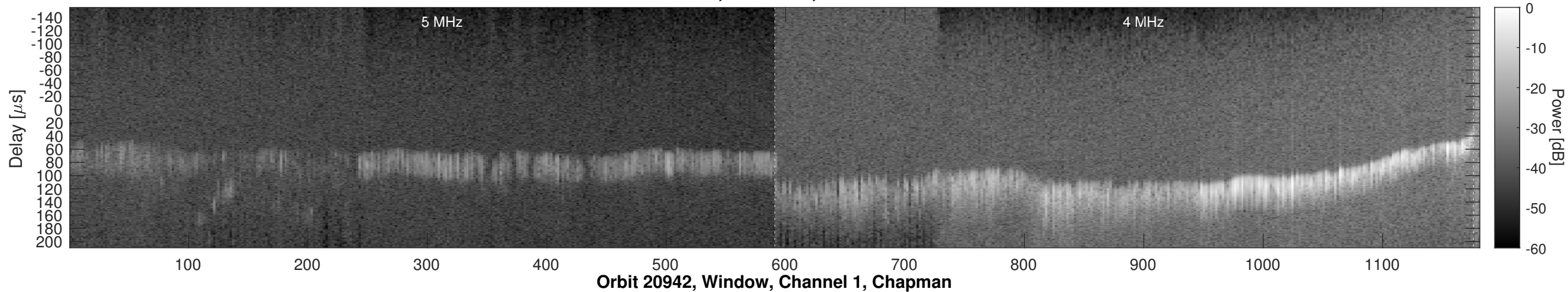
Orbit 20942, Channel 1, Uncorrected
