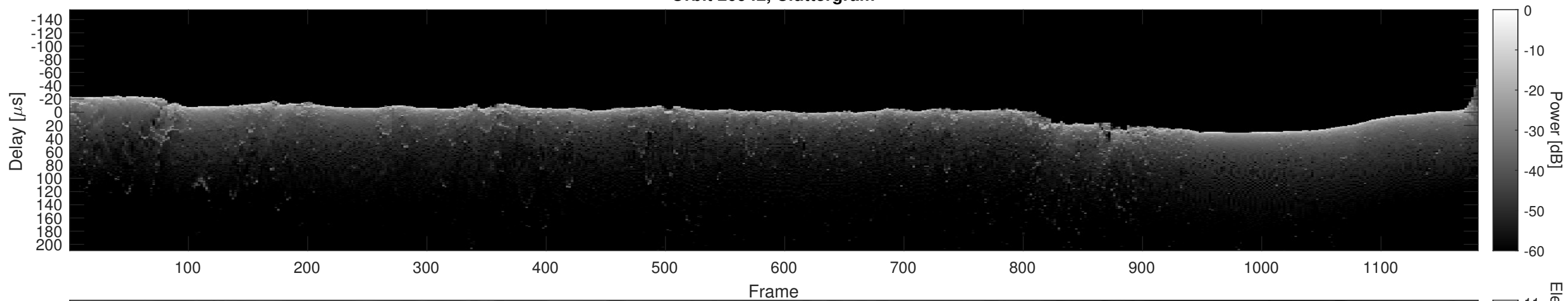
Orbit 20942, Cluttergram
