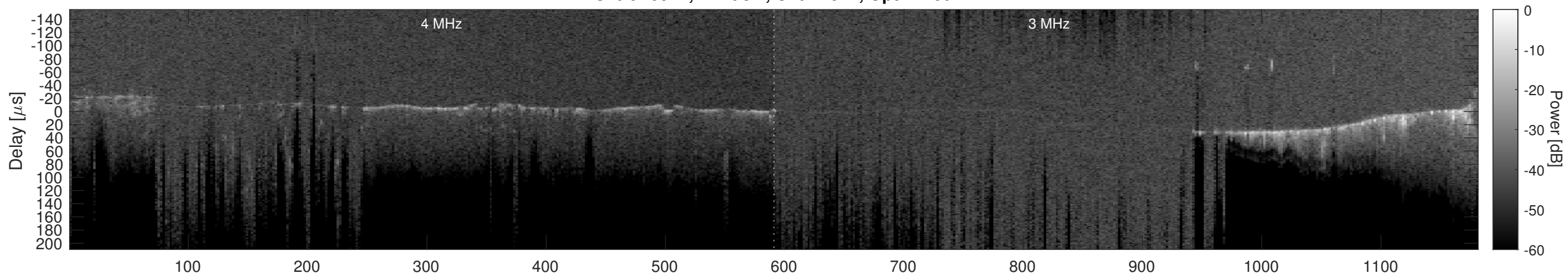
Orbit 20942, Cluttergram
