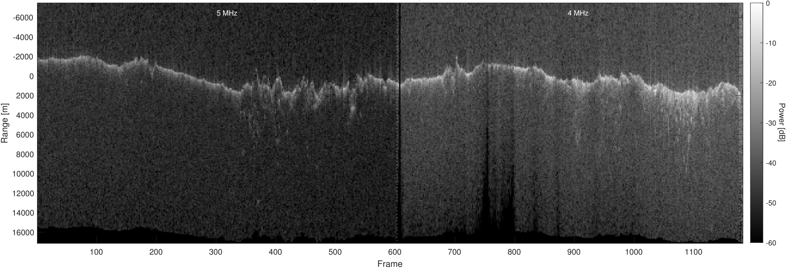
Orbit 20943, Optimized, No Window, Depth-Corrected, Channel 2
