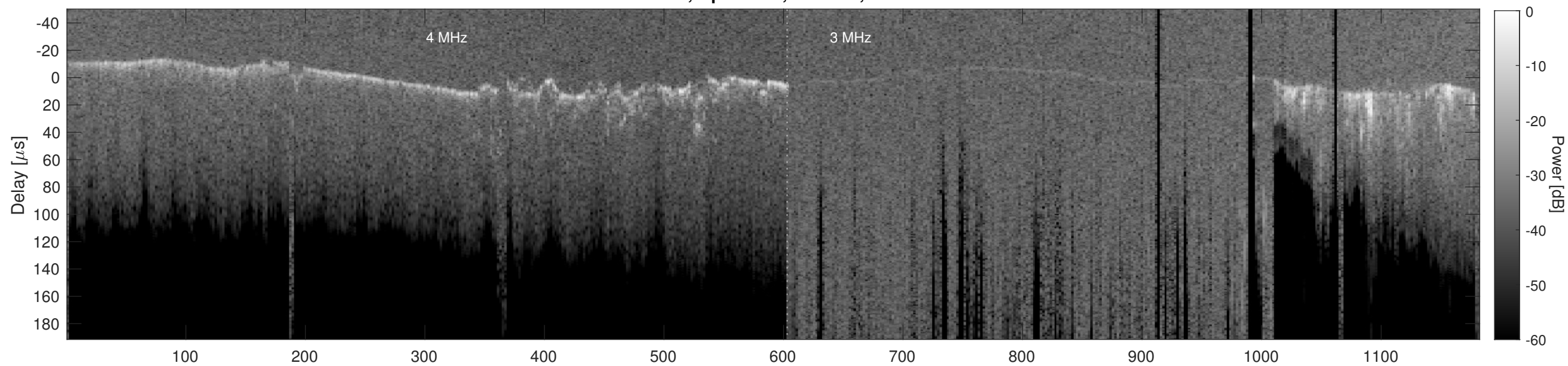
Orbit 20943, Cluttergram
