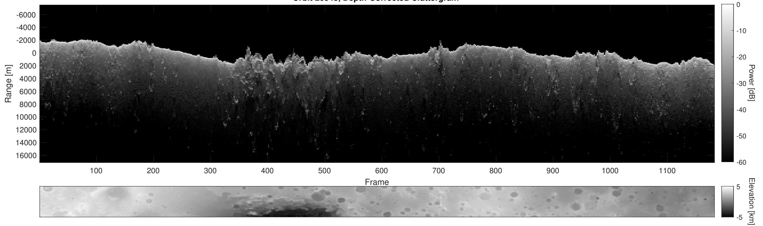
Orbit 20943, Depth-Corrected Cluttergram
