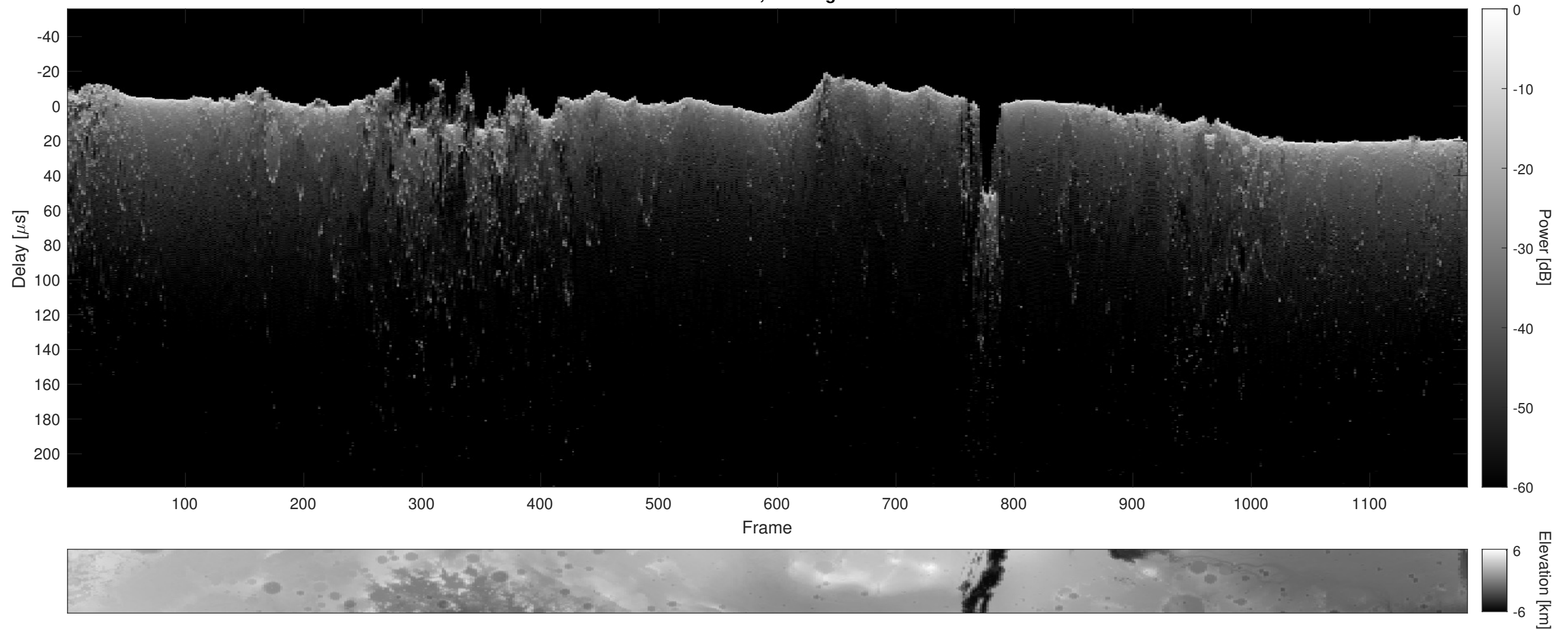
Orbit 20944, Cluttergram
