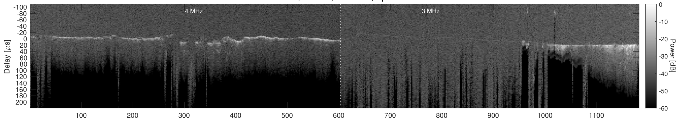
Orbit 20944, Cluttergram
