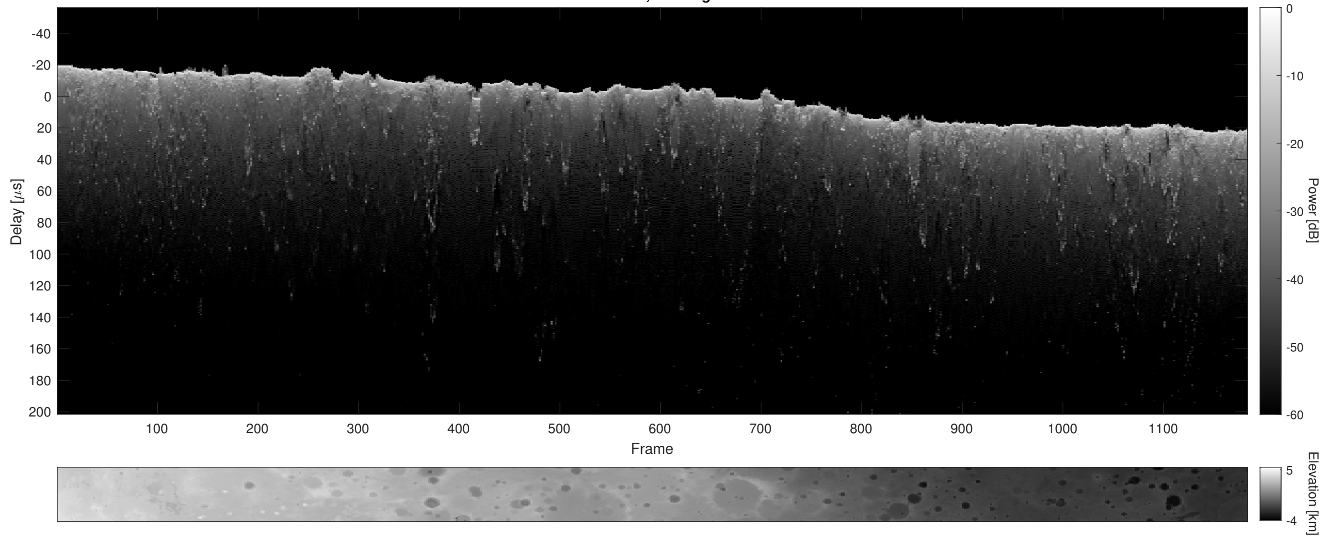
Orbit 20954, Cluttergram
