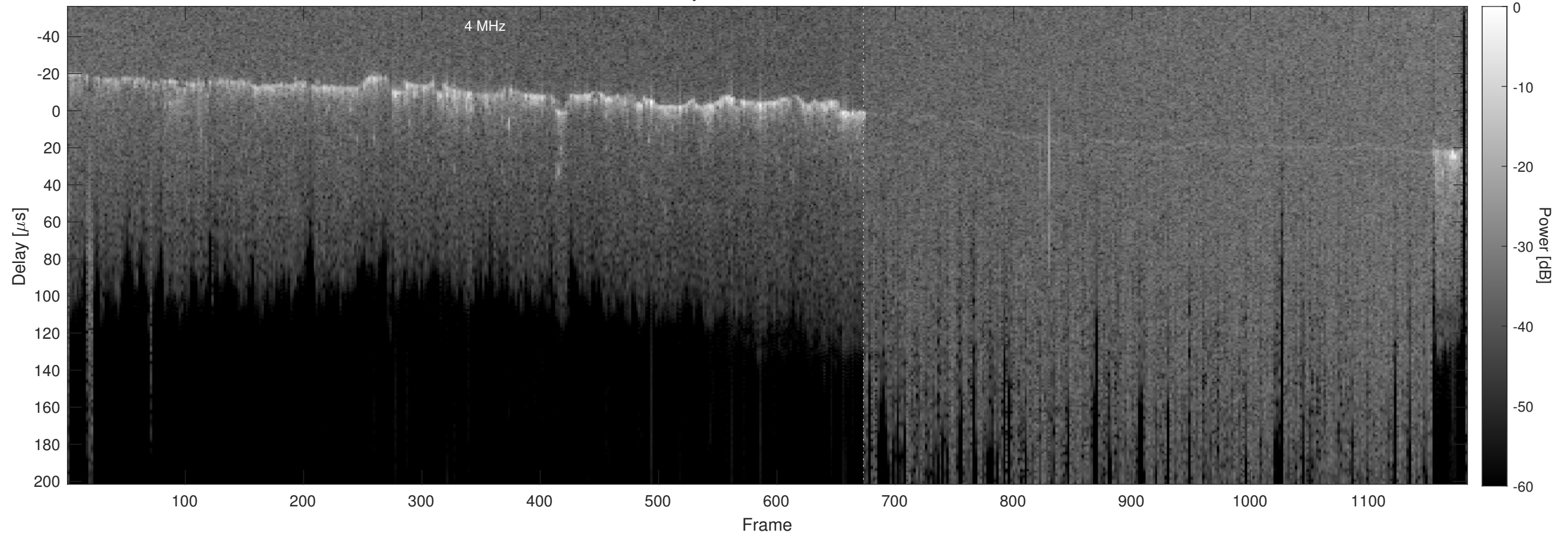
Orbit 20954, Optimized, No Window, Channel 2
