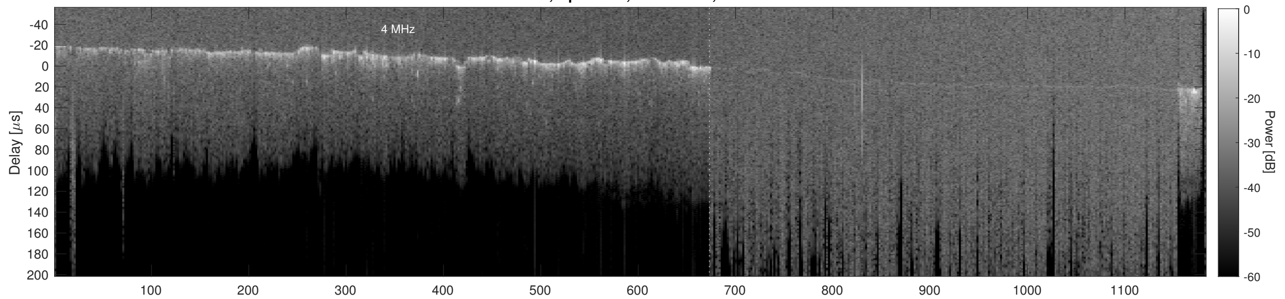
Orbit 20954, Cluttergram
