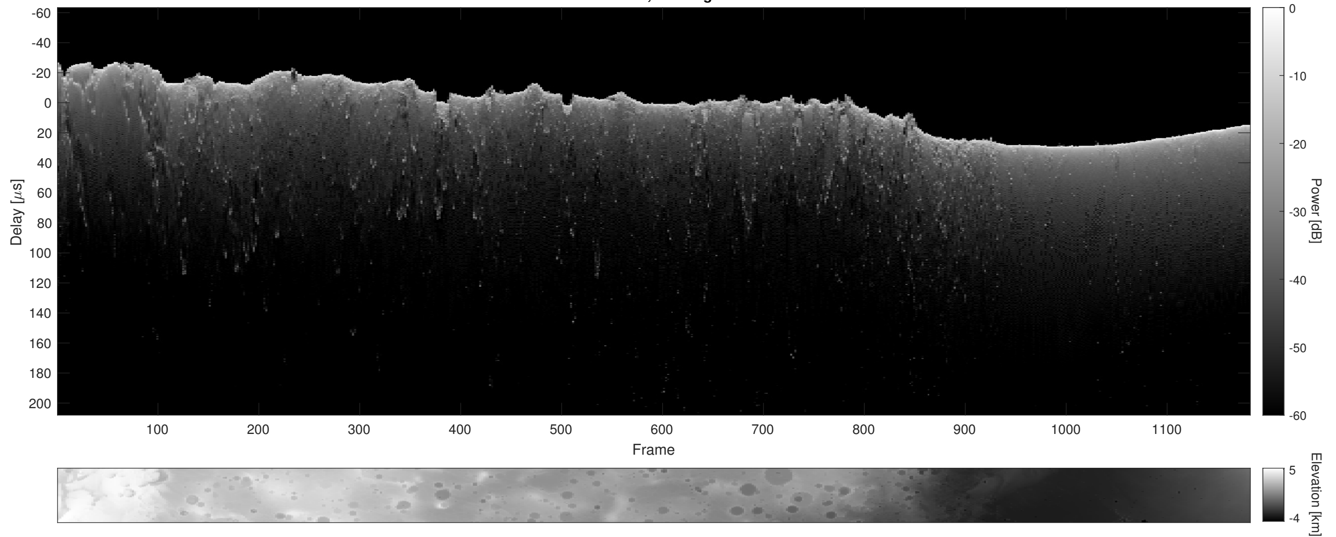
Orbit 20956, Cluttergram
