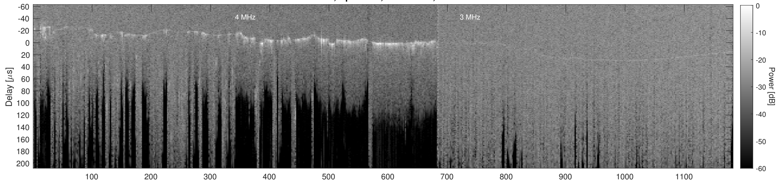
Orbit 20956, Cluttergram
