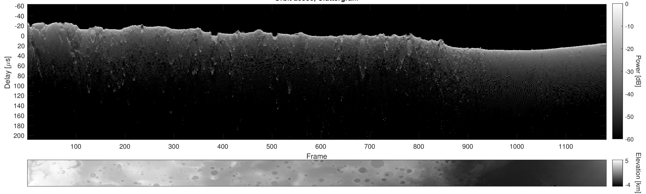
Orbit 20956, Cluttergram
