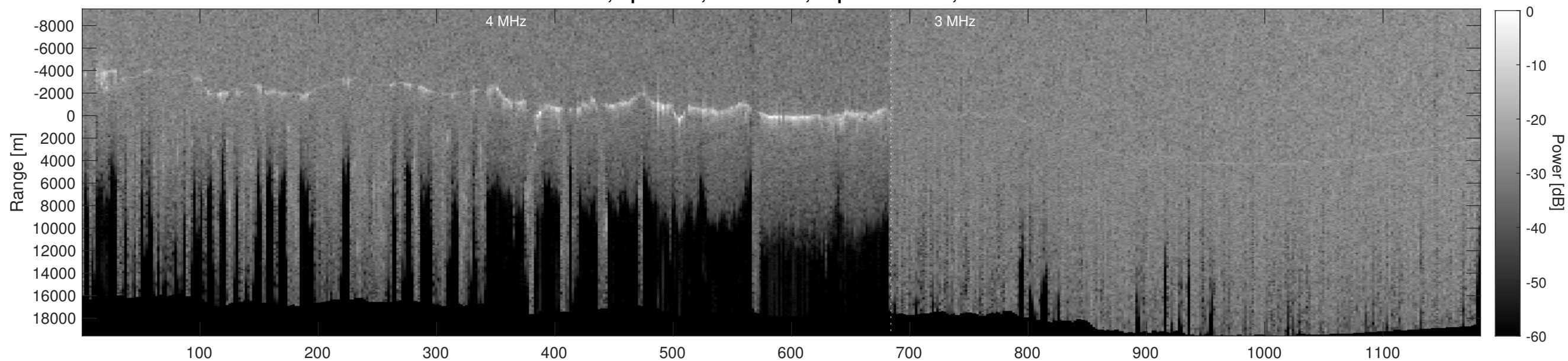
Orbit 20956, Depth-Corrected Cluttergram
