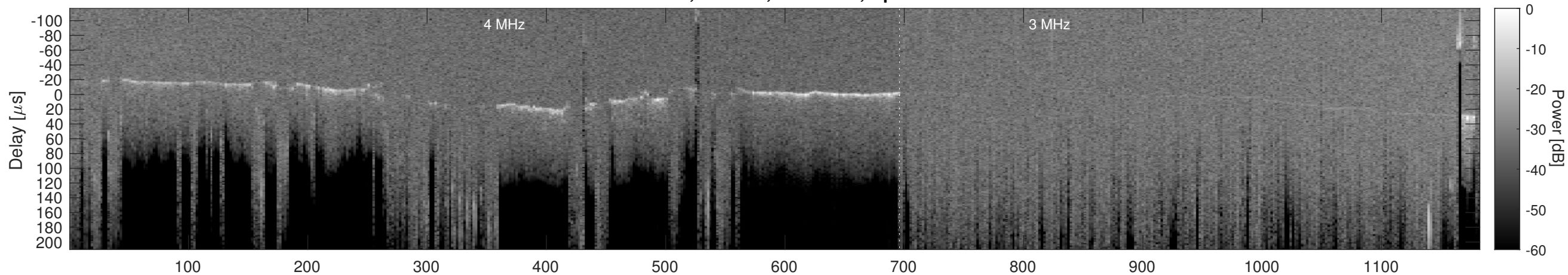
Orbit 20958, Cluttergram
