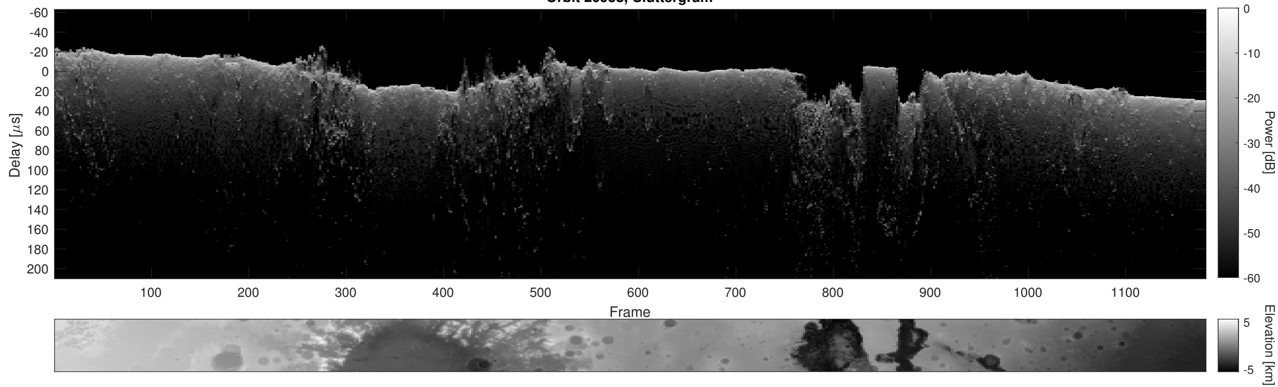
Orbit 20958, Cluttergram
