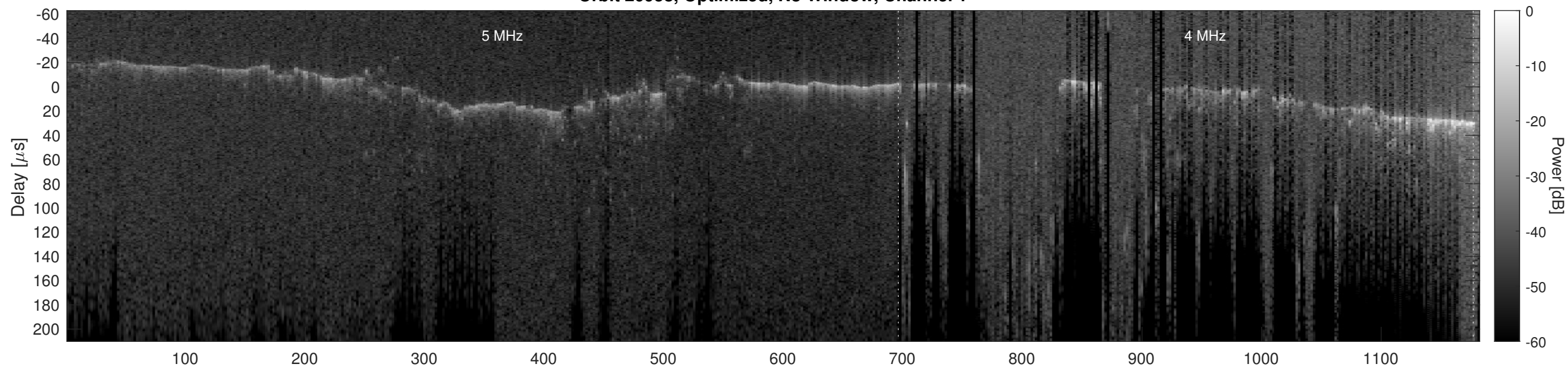
Orbit 20958, Optimized, No Window, Channel 2
