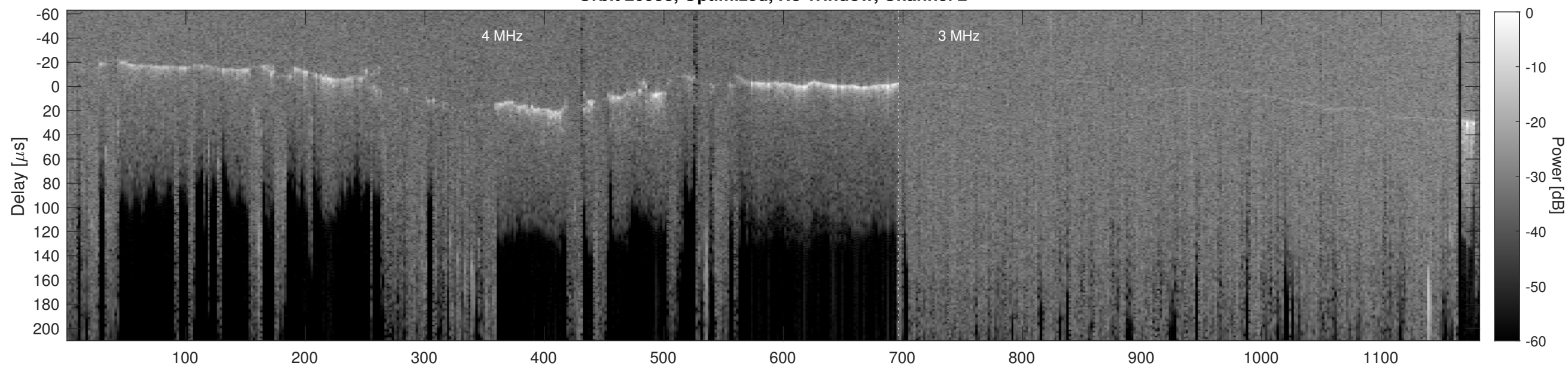
Orbit 20958, Cluttergram
