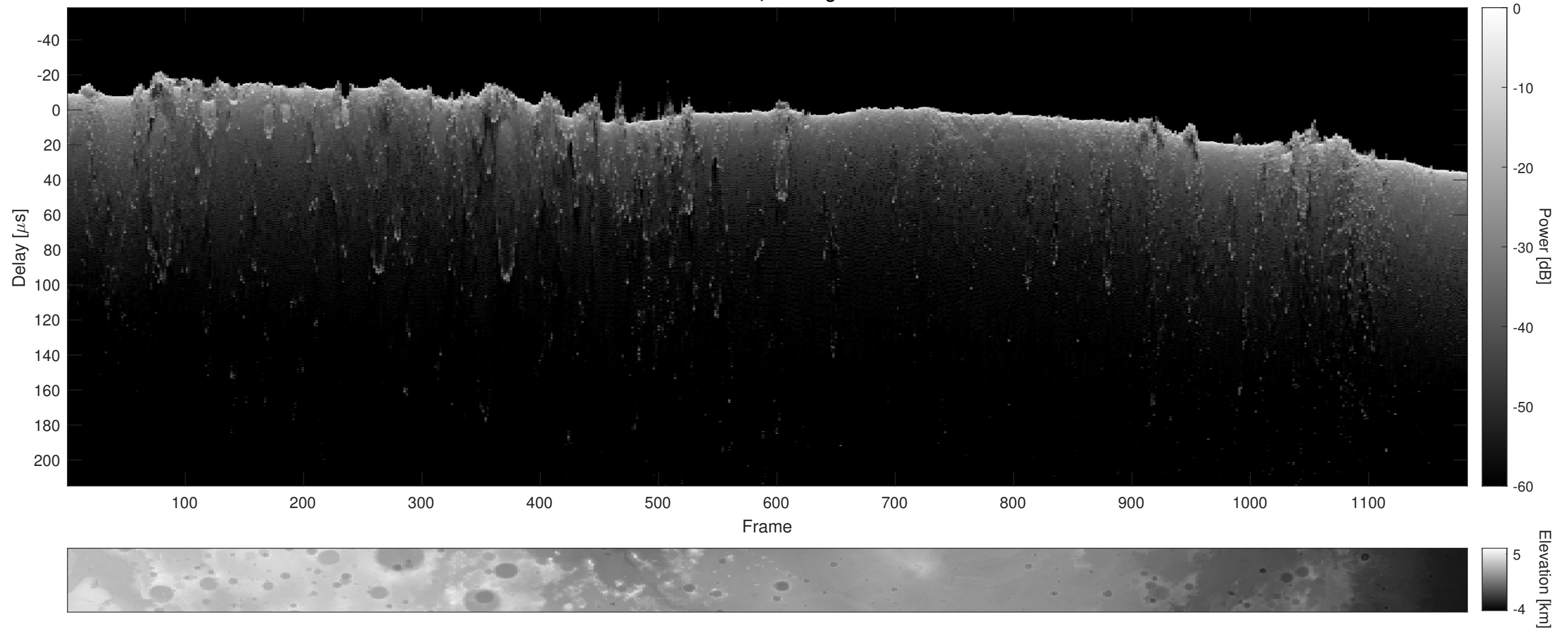
Orbit 20960, Cluttergram
