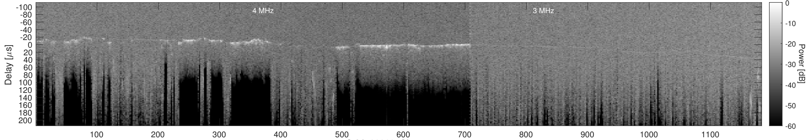
Orbit 20960, Cluttergram
