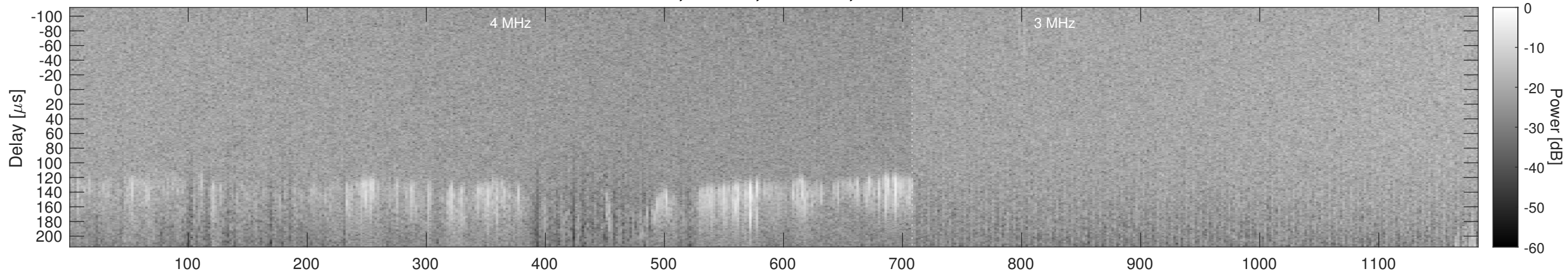
Orbit 20960, Window, Channel 2, Chapman
