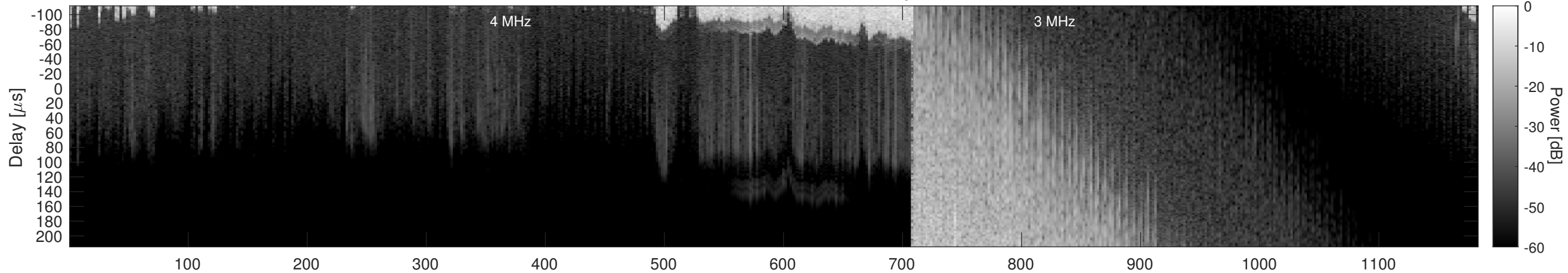
Orbit 20960, Window, Channel 2, Optimized
