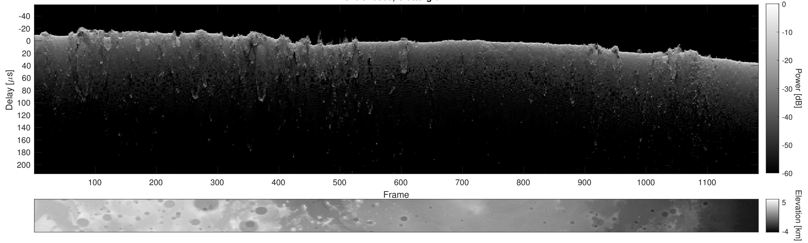
Orbit 20960, Cluttergram
