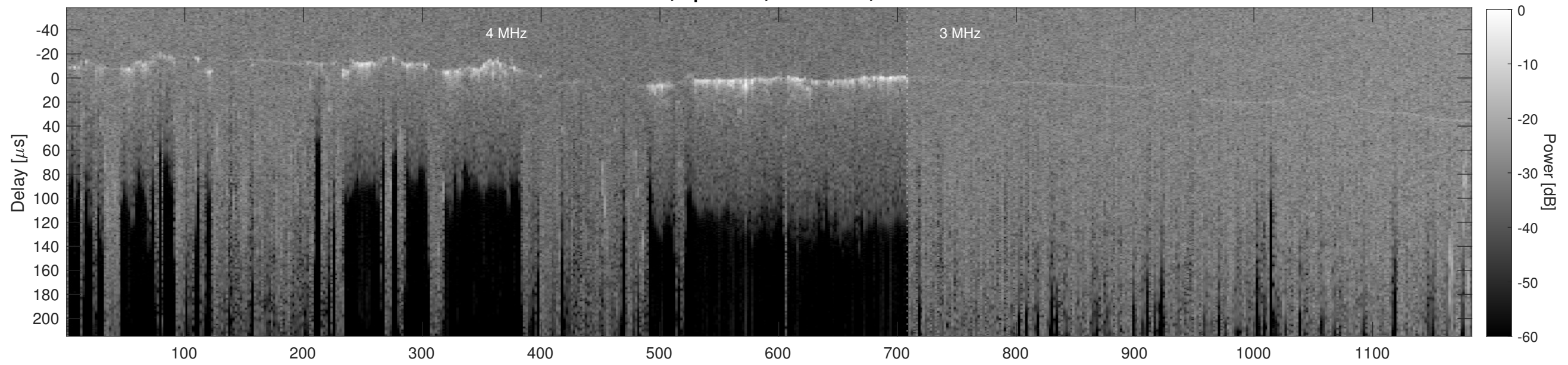
Orbit 20960, Cluttergram
