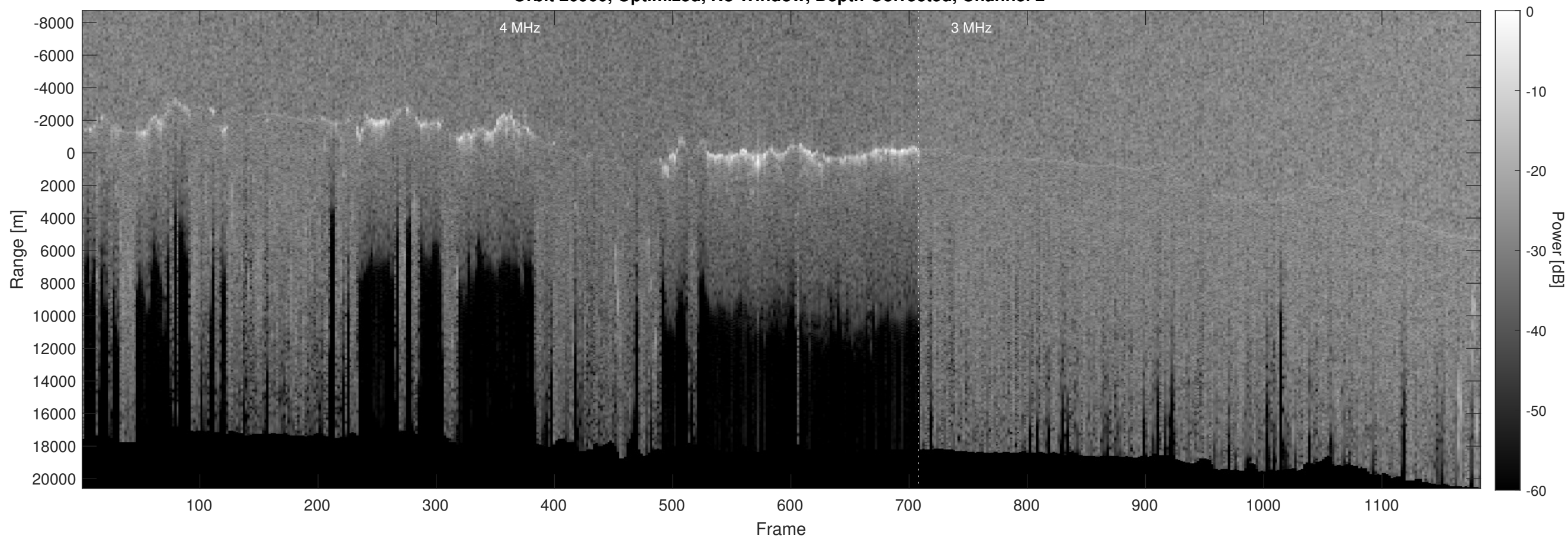
Orbit 20960, Optimized, No Window, Depth-Corrected, Channel 2
