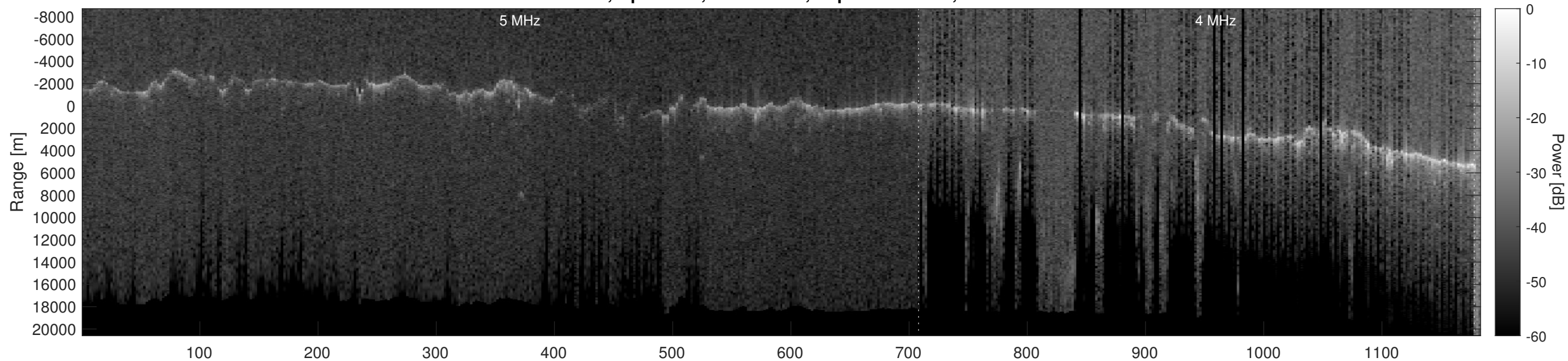
Orbit 20960, Optimized, No Window, Depth-Corrected, Channel 2
