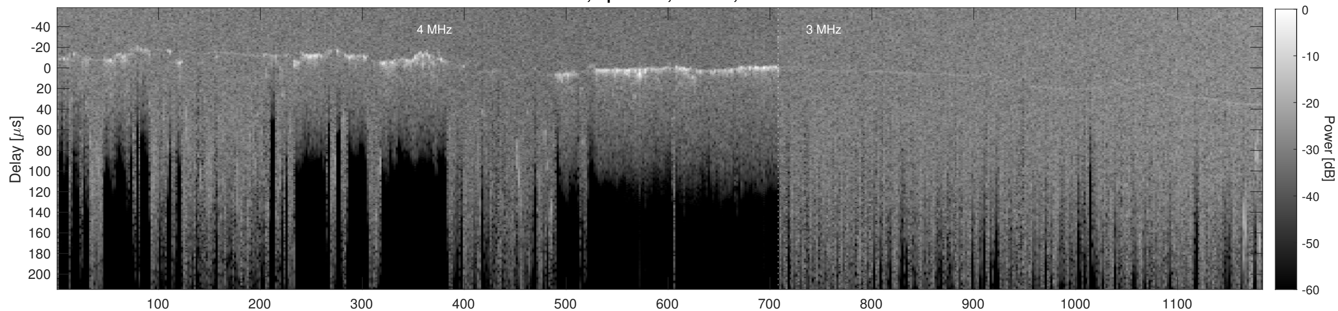
Orbit 20960, Cluttergram
