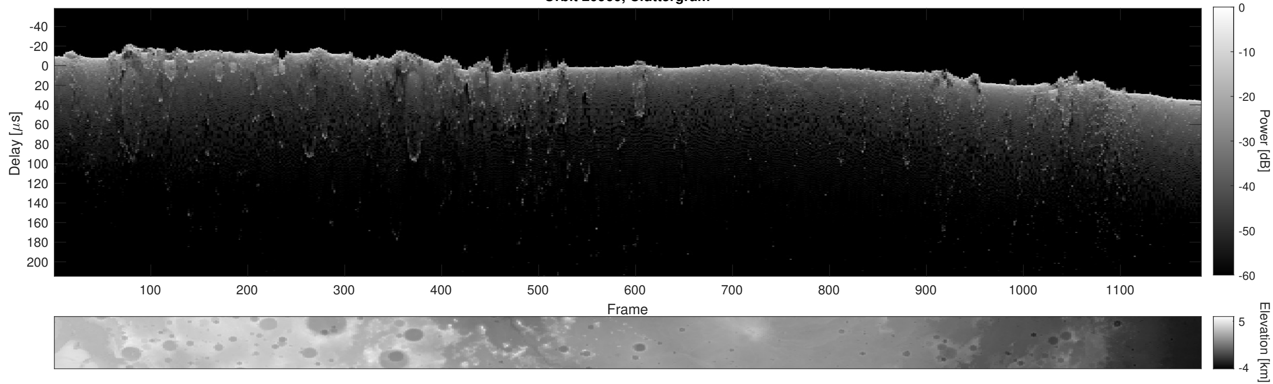
Orbit 20960, Cluttergram
