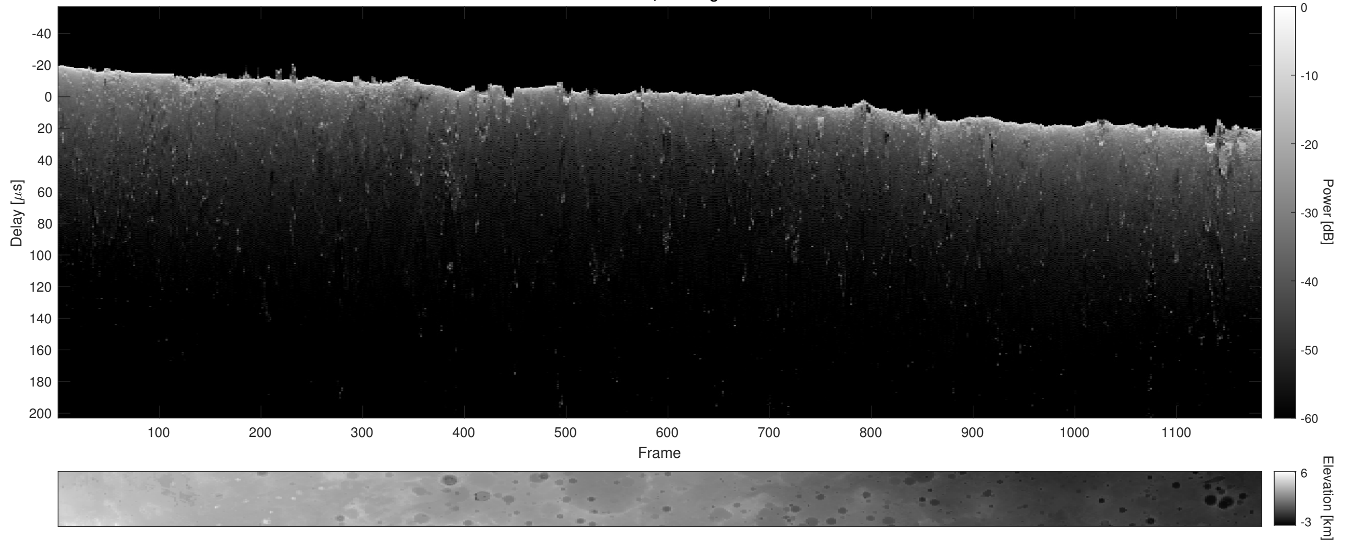
Orbit 20961, Cluttergram
