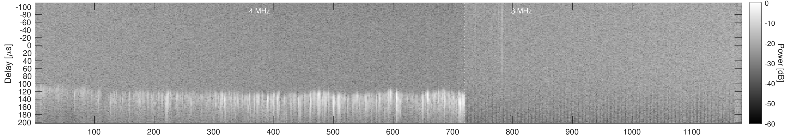
Orbit 20961, Window, Channel 2, Chapman
