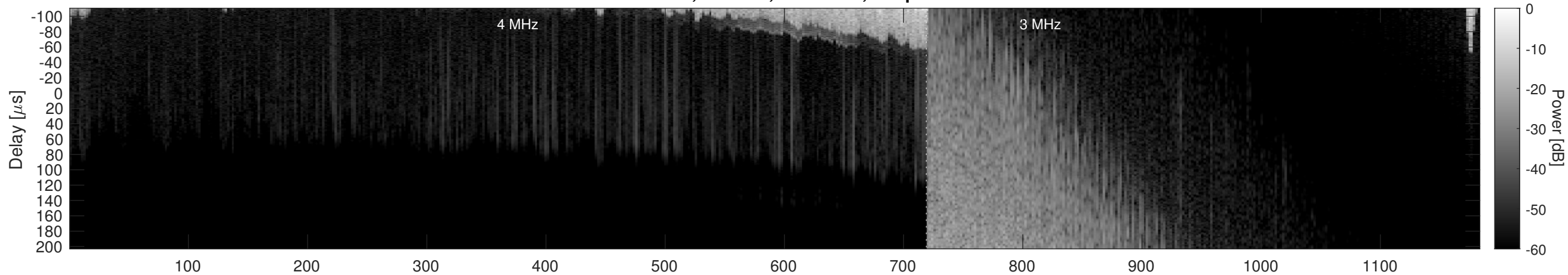
Orbit 20961, Window, Channel 2, Optimized
