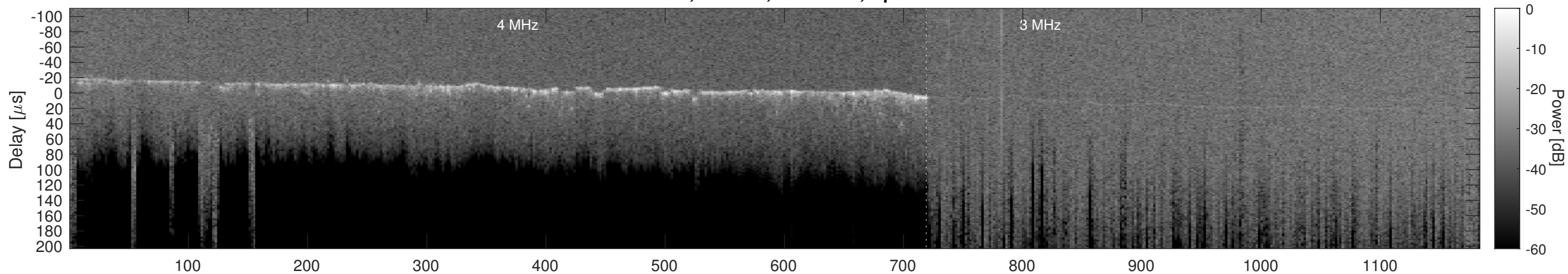
Orbit 20961, Cluttergram
