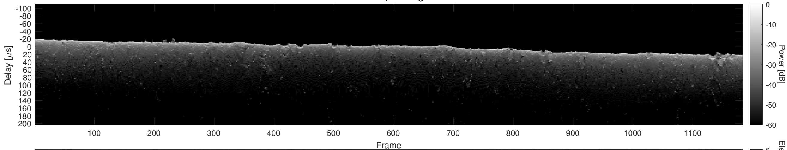
Orbit 20961, Cluttergram
