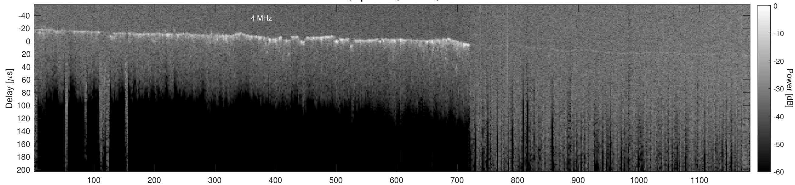
Orbit 20961, Cluttergram
