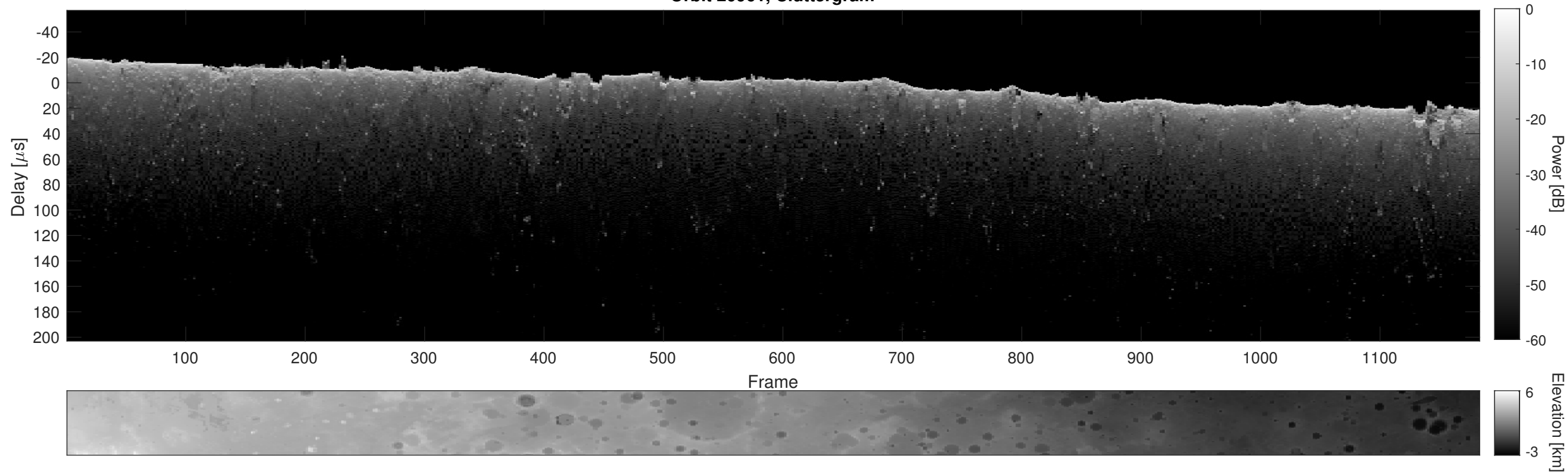
Orbit 20961, Cluttergram
