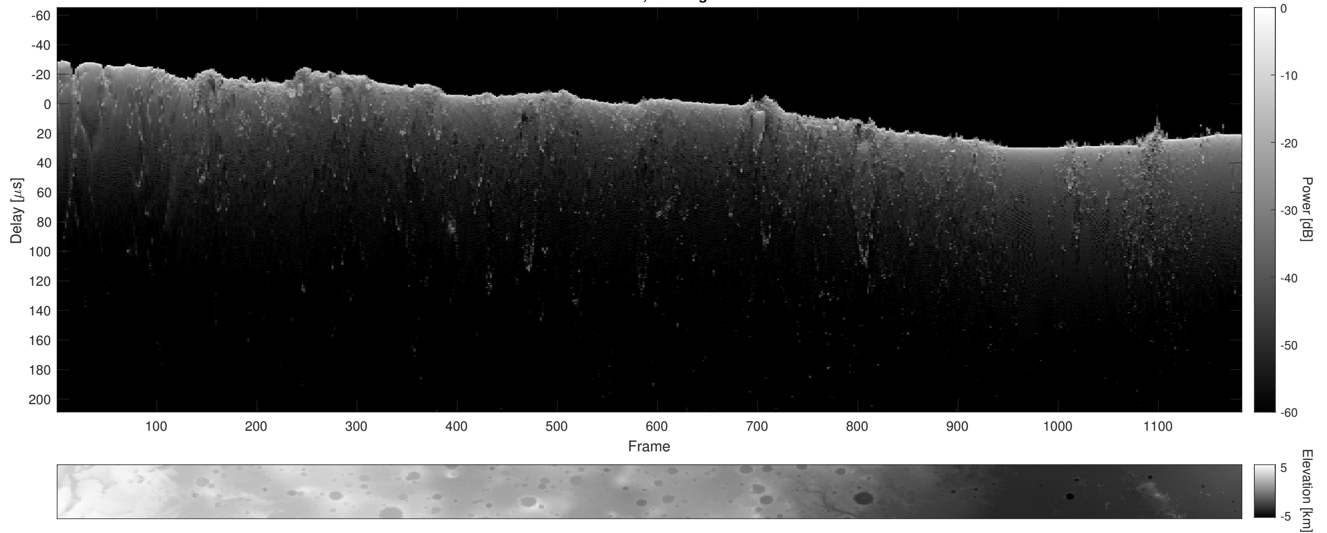
Orbit 20963, Cluttergram
