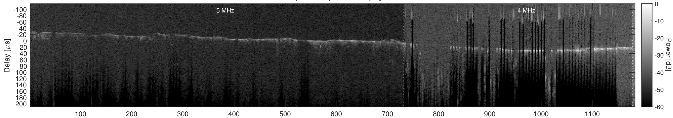
Orbit 20963, Cluttergram
