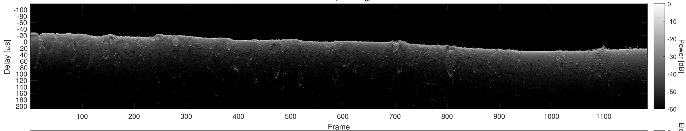
Orbit 20963, Cluttergram
