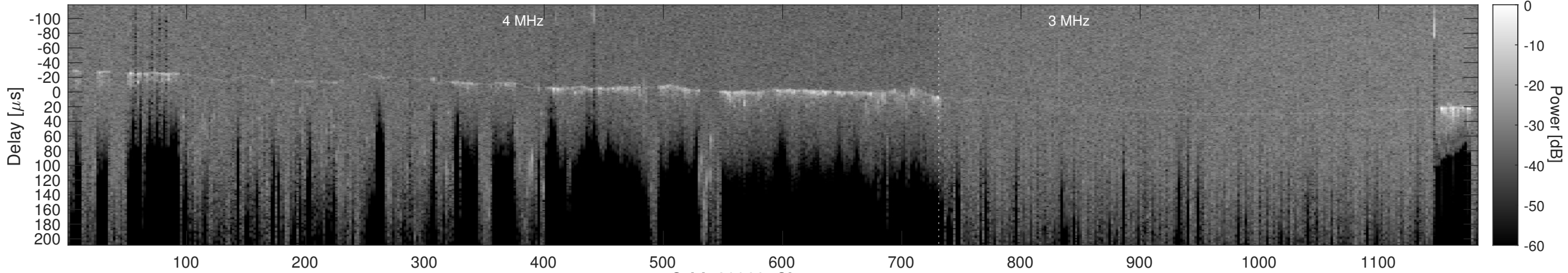
Orbit 20963, Cluttergram
