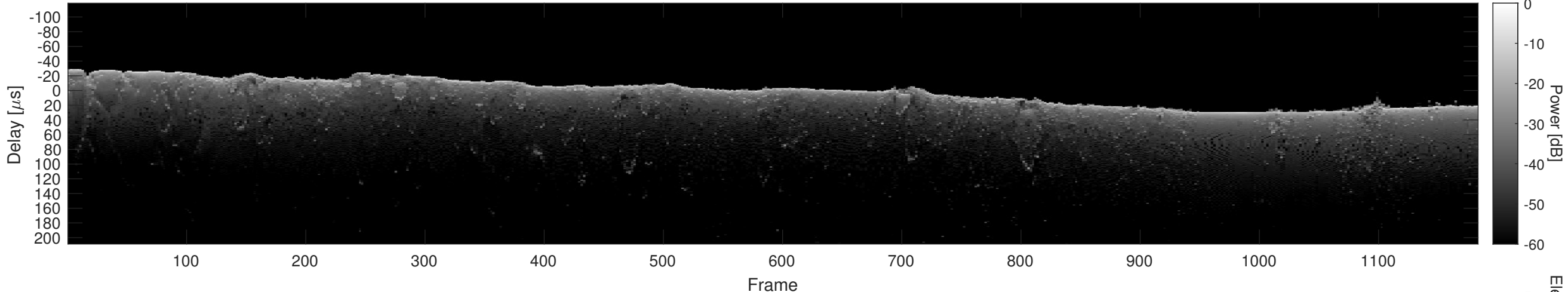
Orbit 20963, Cluttergram
