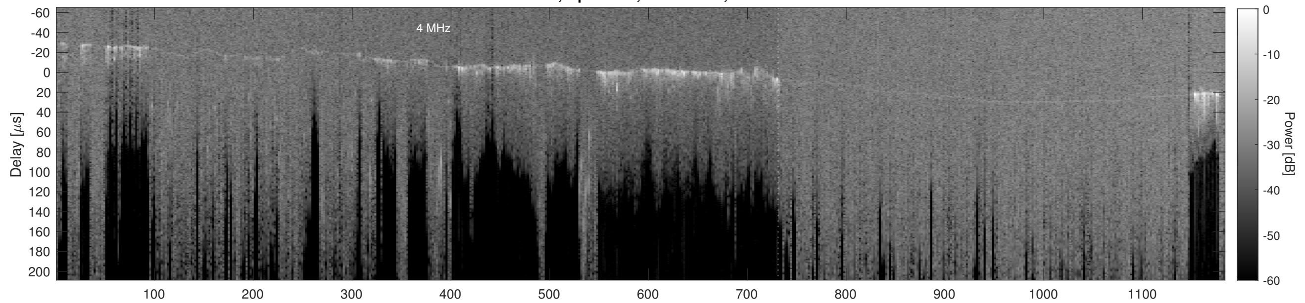
Orbit 20963, Cluttergram
