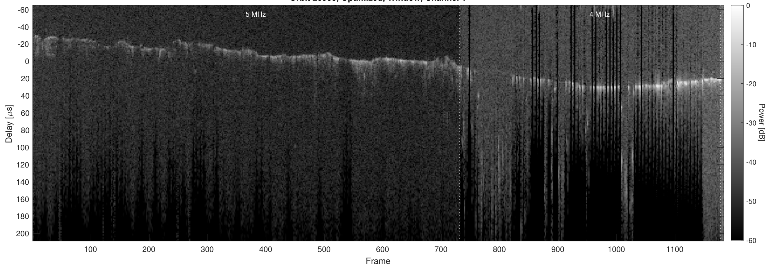
Orbit 20963, Optimized, Window, Channel 2
