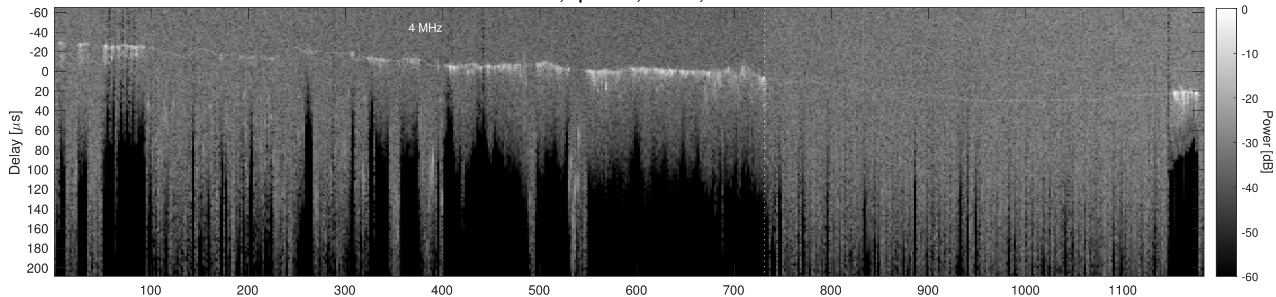
Orbit 20963, Cluttergram
