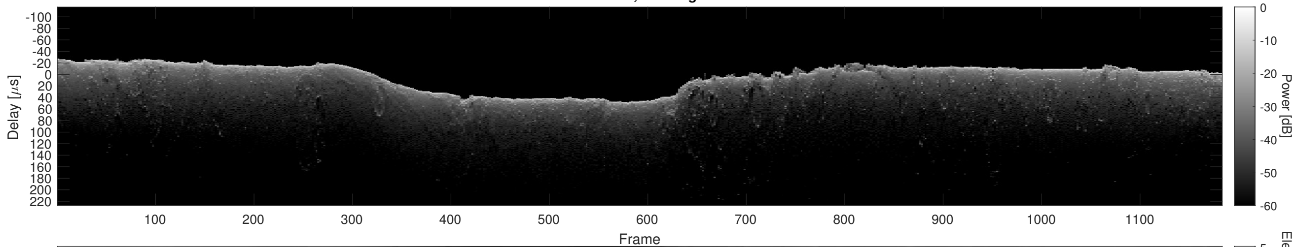
Orbit 20964, Cluttergram
