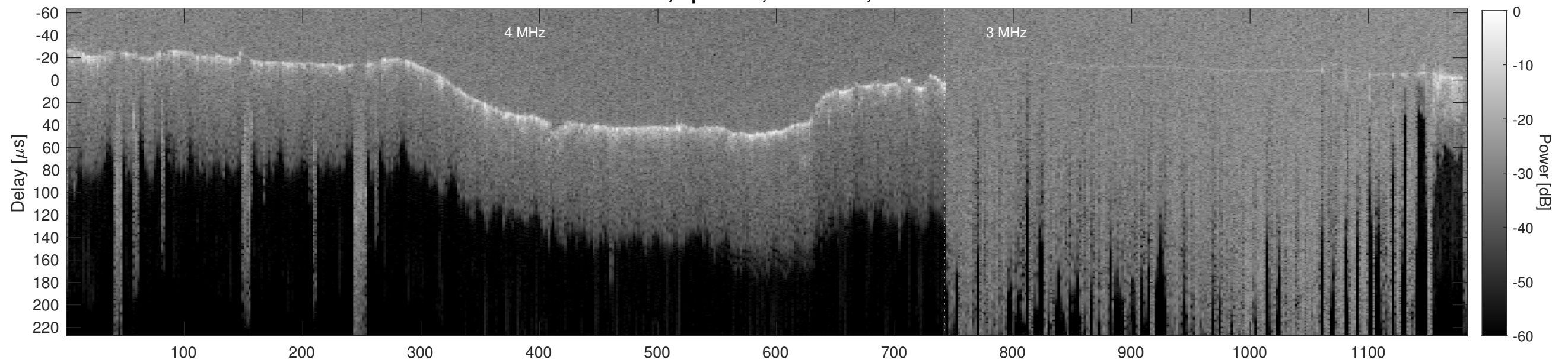
Orbit 20964, Cluttergram
