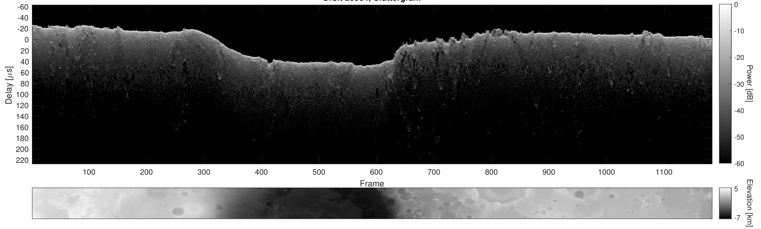
Orbit 20964, Cluttergram
